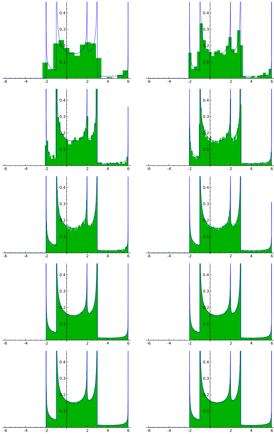
Figure 1: a_2 density function for Sato-Tate group T and a_2(\mathbf{p}) histogram for the curve y^2 = x^6 + 6x^5 - 20x^4 + 20x^3 - 20x^2 - 8x + 8 over \mathbb{Q}(\sqrt{-2}) for \|\mathbf{p}\| \leq 2^N , with N = 12, 14, \dots, 30 .
