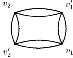
Figure 1. Dual graph of M_{210} \otimes F_3 .
