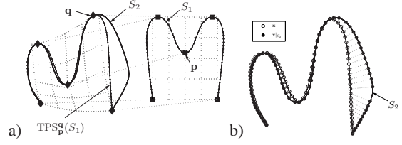
Figure 2: a) TPS wrap of a generic surface based on reduced set of sparse landmarks ( S_1 : original surface, S_2 : target surface, \mathbf{p} : origin landmarks, \mathbf{q} : target landmarks); b) Sticking of the original surface to the target surface after applying the TPS. (see section 4.3)
