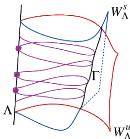
Fig. 3 Illustration of orbits that gain energy by intertwining homoclinic excursions with staying around an invariant manifold.
