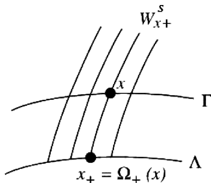
Fig. 5 Illustration of the conditions in (5).
