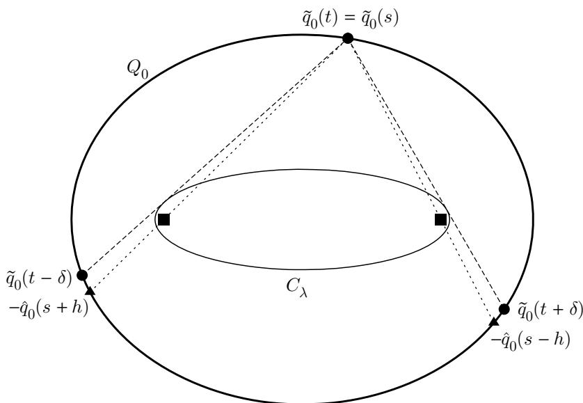
FIGURE 1. A billiard trajectory (dashed line) tangent to the ellipse C_\lambda tends to a billiard trajectory (dotted line) through the foci (the two solid squares) as \lambda \rightarrow b^- . The values of t and s are chosen in such a way that \tilde{q}_0(t) = \hat{q}_0(s) .
