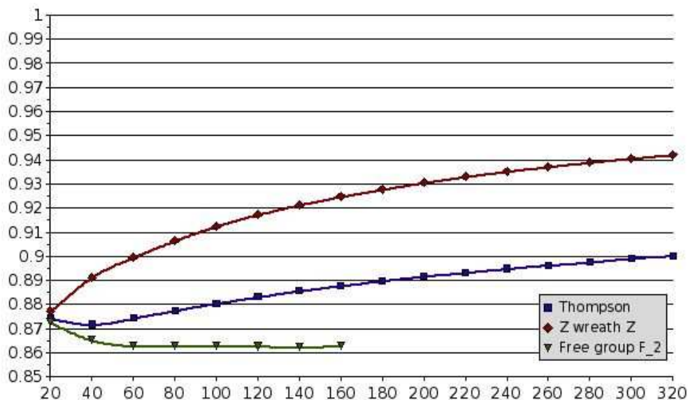
FIGURE 1. Comparing cogrowth estimates \sqrt[p]{\widehat{p}(L)} for three groups.
