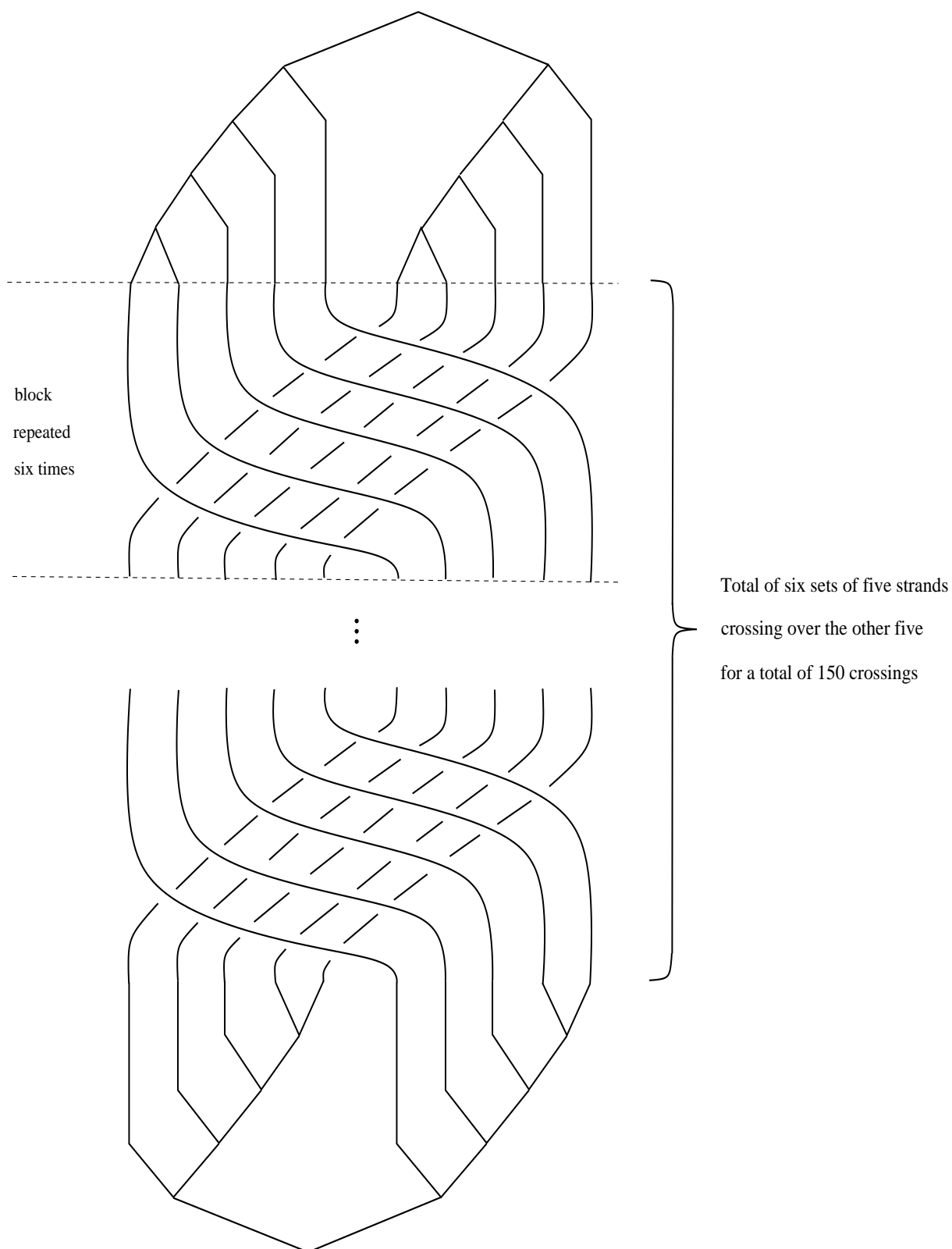
FIGURE 4. The element (x_1\tau_1)^6 , with word length 12, with 9 nodes and 6 blocks where the first 5 strands go over the last 5 strands, giving a total of 150 crossings.
