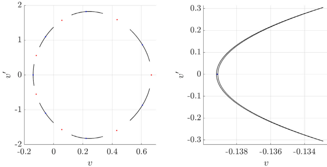
Fig. 11. Left: Intersection with \Sigma = \{u = 0, u' > 0\} of the stable periodic orbit (blue) and the unstable one (red) that have 6 relative maximums in the distance from the first primary for K = 1 and C = 3.5 . In black the first 50 000 intersections of the 6-EC orbit belonging to the B_6^+ with this value of C . Right: Zoom.
