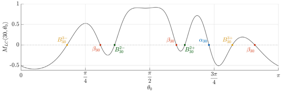
Fig. 20. K = 1 , n = 30 and C = 5 . Curve M_{LC}(30, \theta_0) . In colors the EC orbits and the labels of the families (branches) they belong to.
