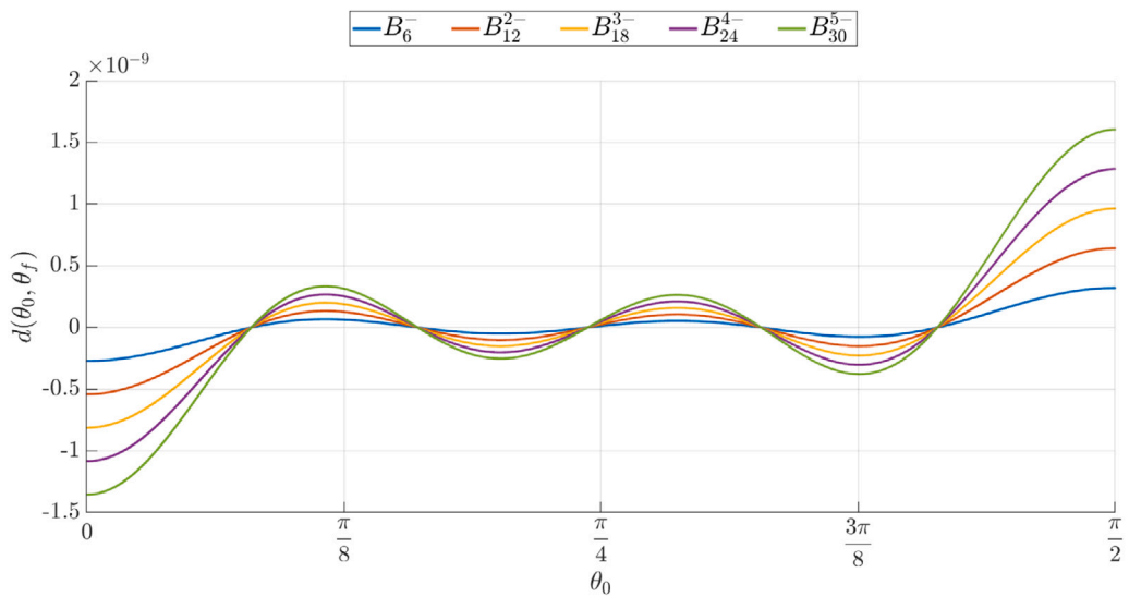
Fig. 17. d(\theta_0, \theta_f) of the orbits of B_{6j}^{j-} for K = 0.1 and j = 1, \dots, 5 .
