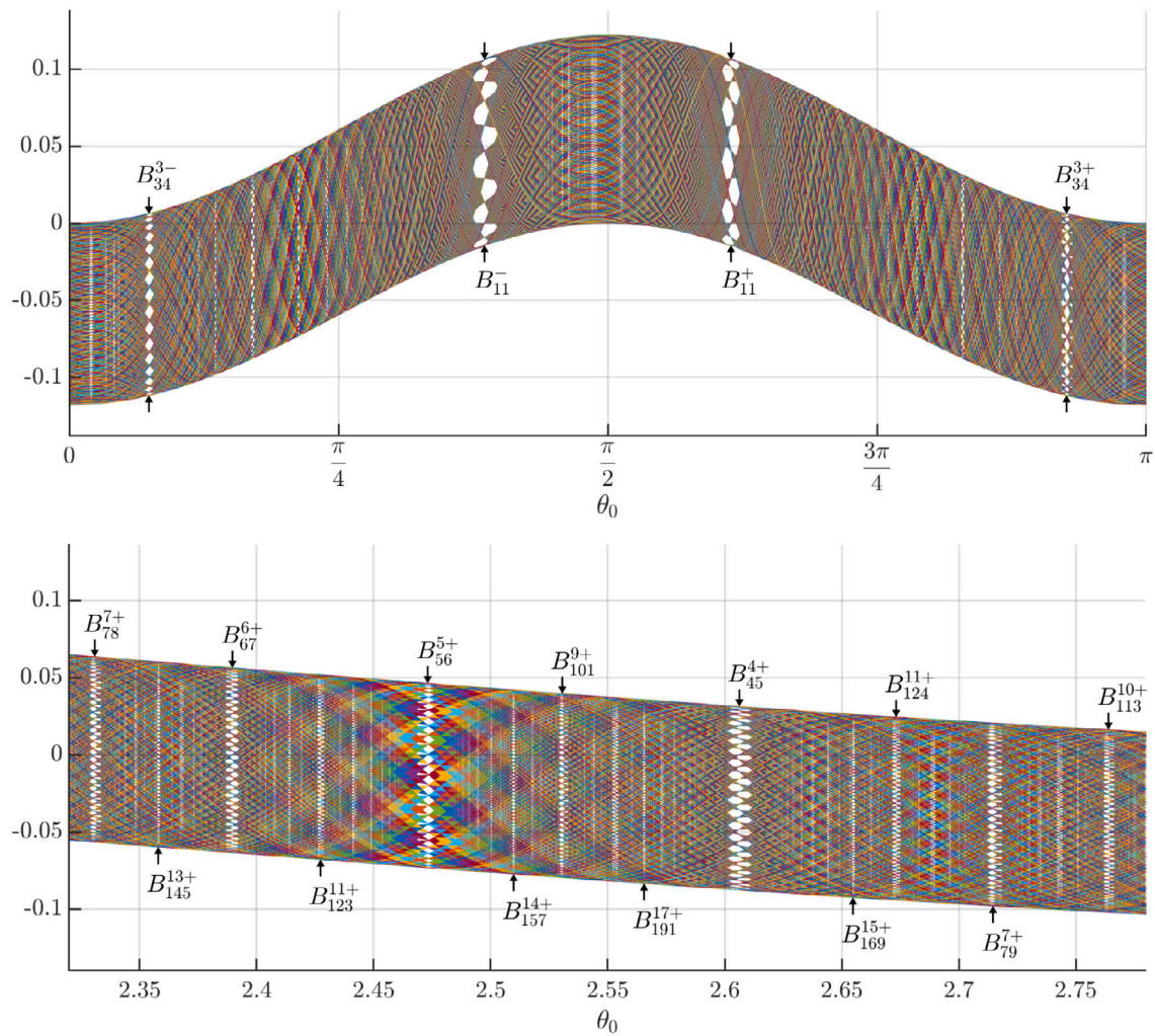
Fig. 22. K = 0.1 . Curves M_{LC}(n, \theta_0) for n = 1, \dots, 1000 and C = 5 . Zoom area. The label B_q^{p\pm} plus an arrow stands for the \theta_0 of an EC orbit belonging to such family.
