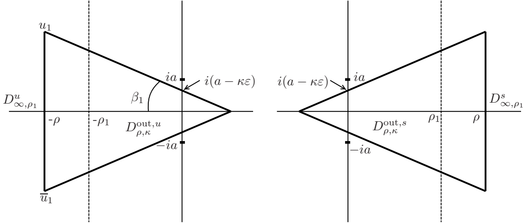
Figure 4: The outer domains D_{\rho, \kappa}^{out, u} and D_{\rho, \kappa}^{out, s} defined in (35).
