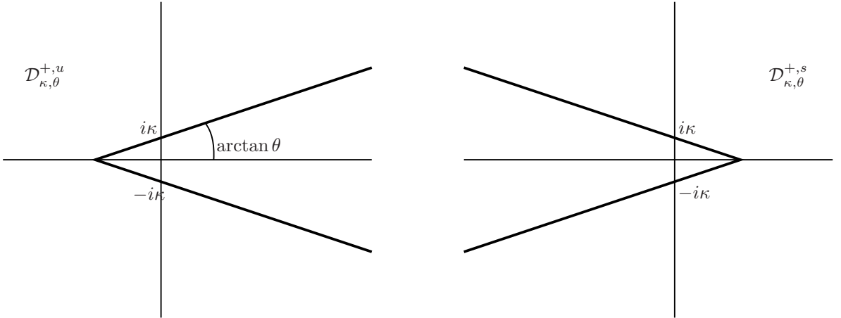
Figure 9: The domains \mathcal{D}_{\kappa, \theta}^{+, u} and \mathcal{D}_{\kappa, \theta}^{+, s} defined in (75).
