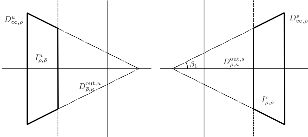
Figure 6: The transition domains I_{\rho, \bar{\rho}}^u and I_{\rho, \bar{\rho}}^s defined in (58).
