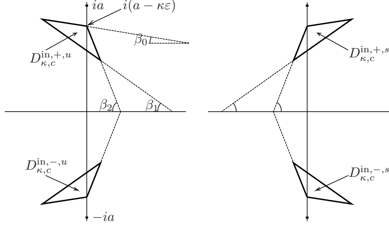
Figure 5: The inner domains defined in (36).
