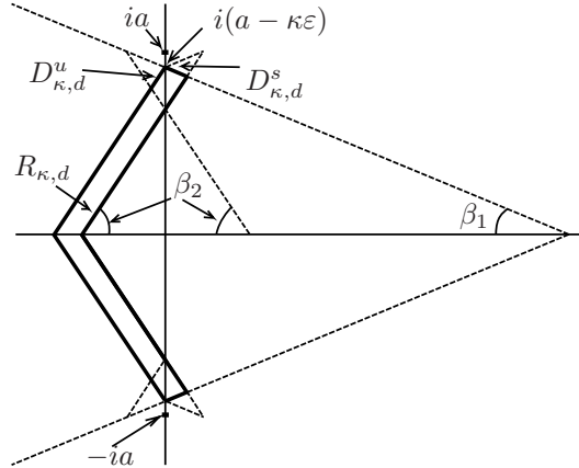
Figure 3: The domain R_{\kappa,d} defined in (33).
