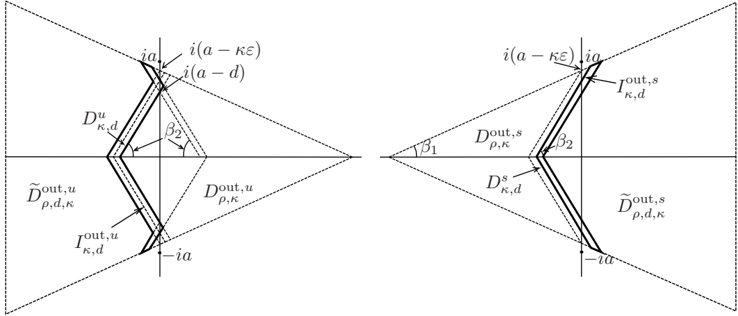
Figure 8: The domains I_{\kappa,d}^{\text{out},u} and I_{\kappa,d}^{\text{out},s} defined in (61).
