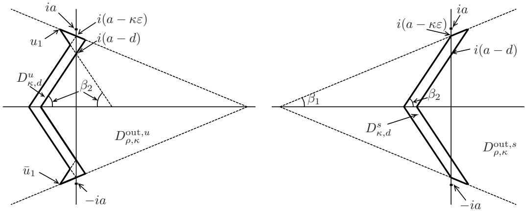
Figure 2: The boomerang domains D_{\kappa,d}^u and D_{\kappa,d}^s defined in (32).
