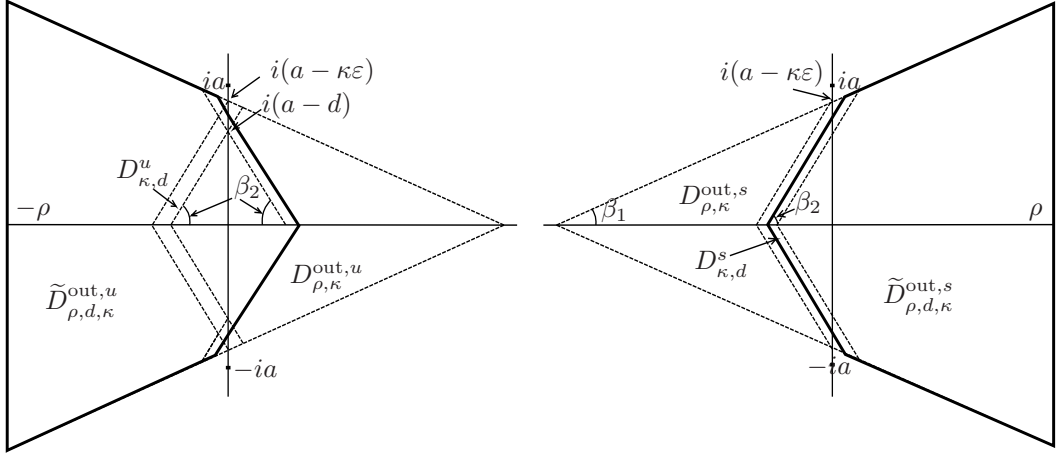
Figure 7: The domains \tilde{D}_{\rho,d,\kappa}^{\text{out},u} and \tilde{D}_{\rho,d,\kappa}^{\text{out},s} defined in (60).
