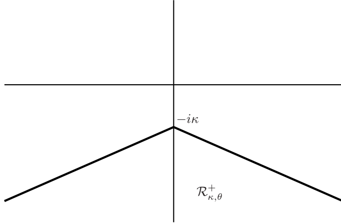
Figure 10: The domain \mathcal{R}_{\kappa, \theta}^+ defined in (76).
