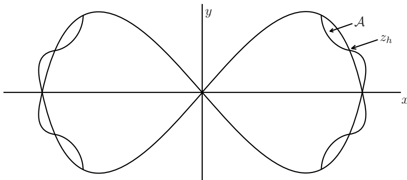
Figure 1: Splitting of separatrices.
