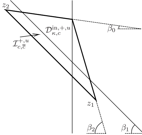
Figure 11: The inner domain \mathcal{D}_{\kappa, c}^{\text{in}, +, u} defined in (70) and the transition domain \mathcal{I}_{c, \bar{c}}^{+, u} defined in (260).
