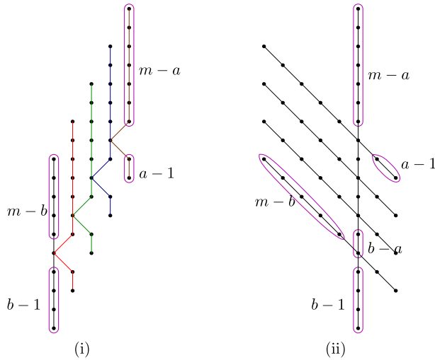
Fig. 1. Two drawings of the unique poset in \mathcal{P}_n^\sigma for a non-overlapping pattern \sigma \in S_m with \sigma_1 = a and \sigma_m = b .
