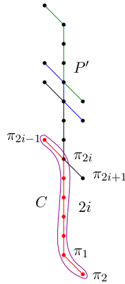
Fig. 6. A generic poset in \mathcal{P}^{2143} .
