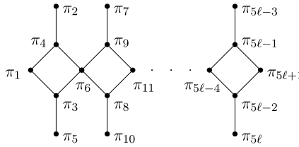
Fig. 7. A poset in \mathcal{P}^{2413} .
