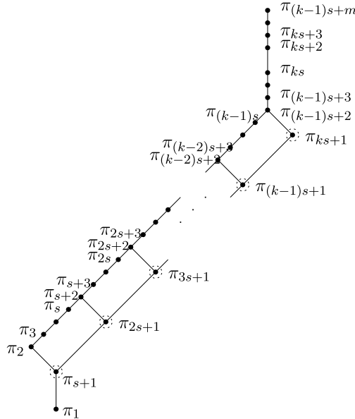
Fig. 3. The poset Q_k in \mathcal{P}^{134\dots(s+1)2(s+2)(s+3)\dots m} corresponding to dense k -clusters. In this picture, s = 5 and m = 10 .
