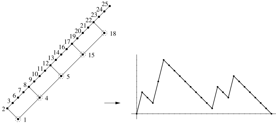
Fig. 4. An example of the bijection between linear extensions of \tilde{Q}_5 and lattice paths, for s = 5 and k = 5 .
