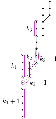
Fig. 5. A generic poset in \mathcal{P}^{1423} .
