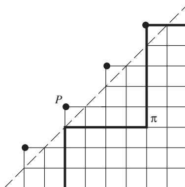
Fig. 1. The path \pi = \underline{E}E\underline{N}N\underline{N}E\underline{E}E\underline{E}E\underline{E}E\underline{N}N\underline{N}N\underline{N}N\underline{E}E not above P = (N^2E^2)^4 . It has i(\pi) = 3 and e(\pi) = 2 , corresponding to the steps underlined.
