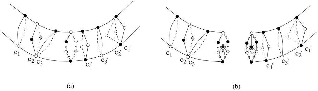
Fig. 1. Cutting along a non-contractible cycle cuts a handle and creates two cylindrical ends.
