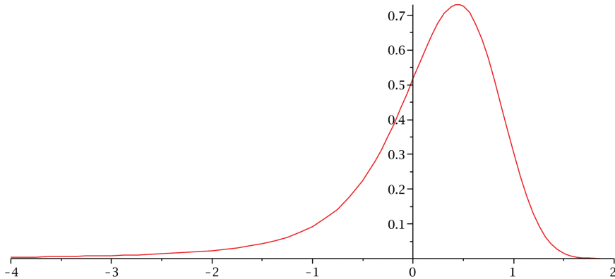
Fig. 3. The airy distribution. [Color figure can be viewed in the online issue, which is available at wileyonlinelibrary.com .]
