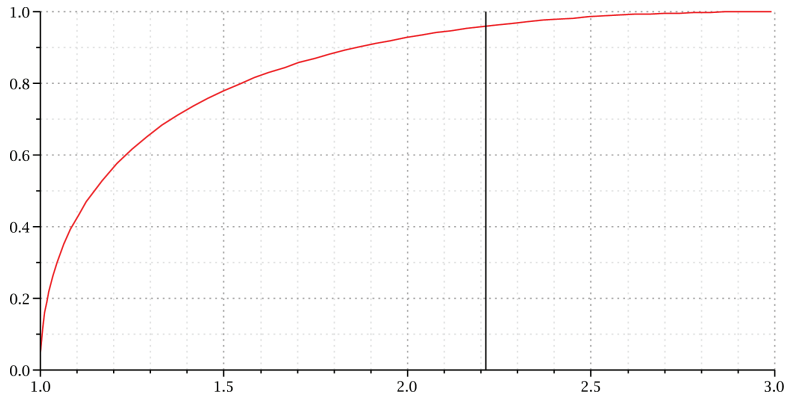
Fig. 4. Size of largest block for planar graphs with \mu n edges, \mu \in (1, 3) . The ordinate gives the value \alpha(\mu) such that the largest block has size \sim \alpha(\mu)n . The value at \kappa is 0.9598 as in Theorem 5.4. [Color figure can be viewed in the online issue, which is available at wileyonlinelibrary.com .]
