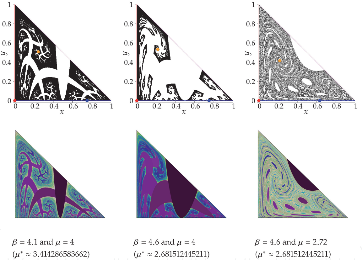
Figure 6. (Top row) The invariant set S_{\mu, \beta} for several values of \beta > 4 and \mu > \mu^*(\beta) . In Figure 4 we can see the location in the parameter space that corresponds to these three dynamical pictures. (Bottom row) Escaping regions with the number of iterates needed to go out of the domain represented in a gradient from 1 (black), 2 (dark violet), 3 (light violet) to 50 (yellow) iterates. Note the fractal nature of the invariant set and of the escaping regions (see movie1.mp4 for an animation of the invariant and escaping sets as a function of model parameters).
