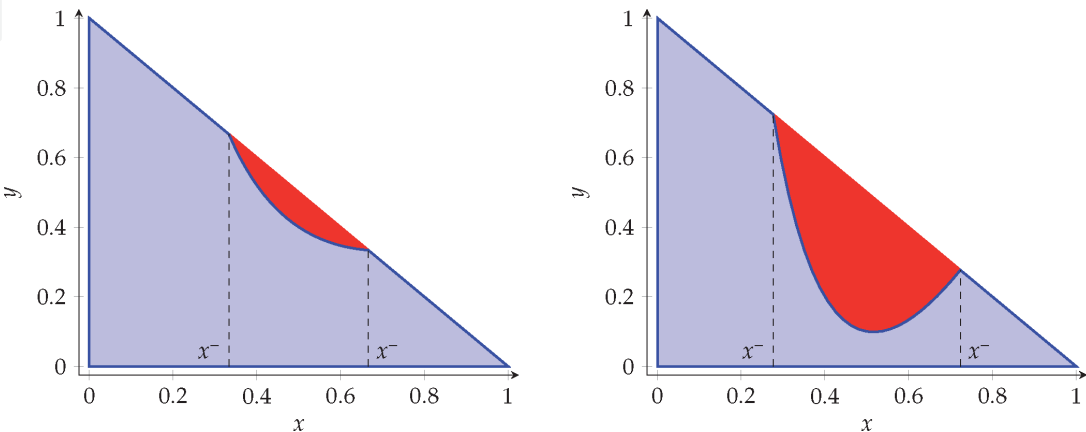
Figure 7. Two examples of the domain S in blue with the one-step escaping set \varepsilon_{\mu,\beta} plotted in red for \beta = 4.5 and \mu = 2 (left picture) and \beta = 5 and \mu = 3.75 (right picture). The one-step escaping set \varepsilon_{\mu,\beta} is vertically delimited by the curves \frac{1-\mu x(1-x)}{(\beta-\mu)x} < 1-x on the interval with endpoints x^\pm := \frac{1}{2} \pm \sqrt{\frac{1}{4} - \frac{1}{\beta}} .
