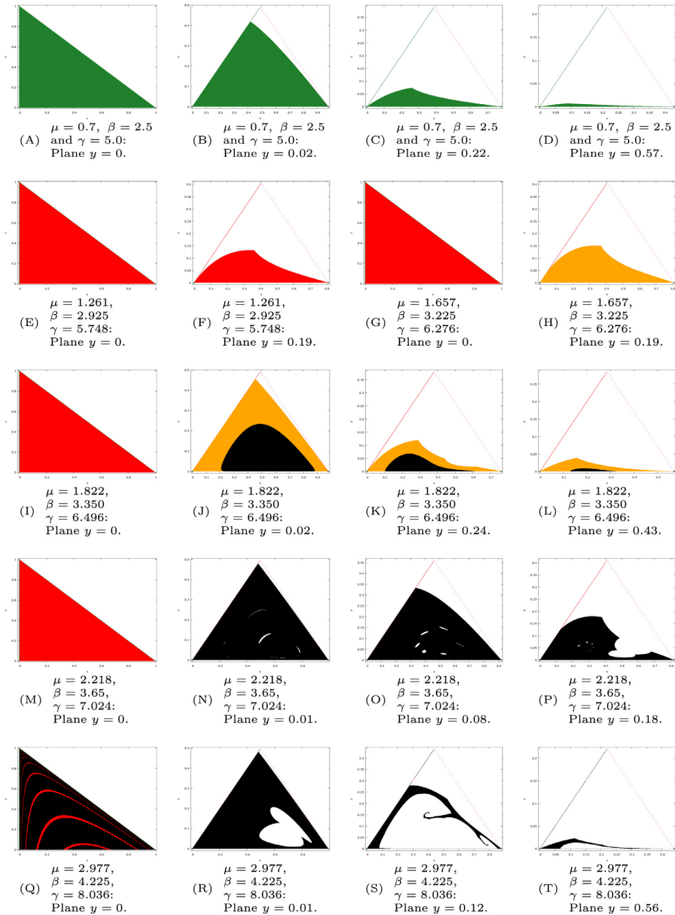
Fig. 2. Plots of the intersection of S with the planes y = \text{cnt} for several choices of the planes and the parameters \mu, \beta and \gamma . Points drawn in dark green color converge to the fixed point (0,0,0) , points in red converge to the fixed point (\frac{\mu-1}{\mu}, 0, 0) , points in orange converge to the fixed point (\beta^{-1}, 1 - \mu^{-1} - \beta^{-1}, 0) , and points in black belong to the invariant set S but do not belong to the basin of attraction of any fixed point. The dashed magenta lines show the boundary of the cut of the plane y = \text{cnt} with the domain \mathcal{E} (which is defined in page 7).
