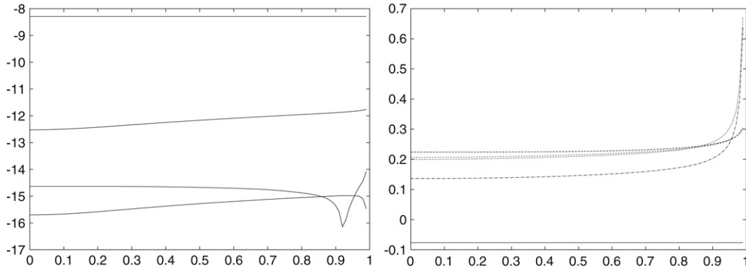
Fig. 2. Left: \log_{10} of the error in the numerical computation of \Delta(\varepsilon) versus \varepsilon for \theta = (\sqrt{5} - 1)/2 . We use formula (19) and the first three extrapolation methods using (38). Right: the coefficients \gamma, A_1^{(\pm 1)}, A_2^{(\pm 1)} of the extrapolation versus \varepsilon .
