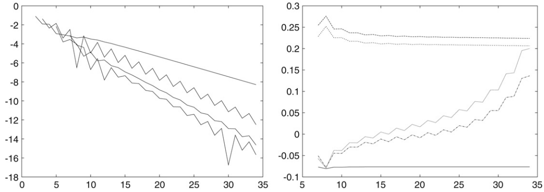
Fig. 3. Left: \log_{10} of the error in the numerical computation of \Delta(0.1) by using the same methods as in Fig. 2, versus the index n of the Fibonacci F_n giving the number of iterates used. Right: the coefficients \gamma, A_1^{(\pm 1)}, A_2^{(\pm 1)} of the extrapolation versus n .
