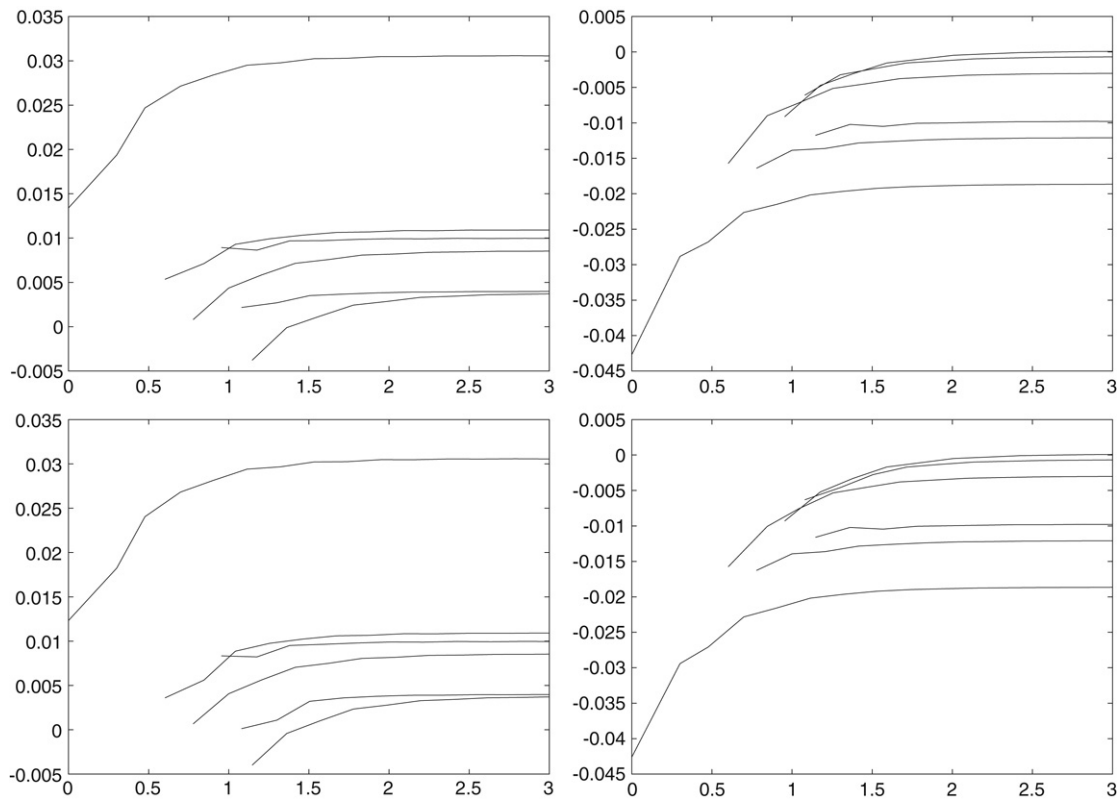
Fig. 5. The two plots on the top correspond to \varepsilon = 0 and those on the bottom to \varepsilon = 0.5 . Left: (-1)^n F_n^j \cdot \text{Re}(\hat{\xi}_{F_n^j}) versus \log_{10} F_n^j, j = 1, \dots, 6 . Right: F_n^j \cdot \text{Im}(\hat{\xi}_{F_n^j}) versus \log_{10} F_n^j, j = 1, \dots, 6 .
