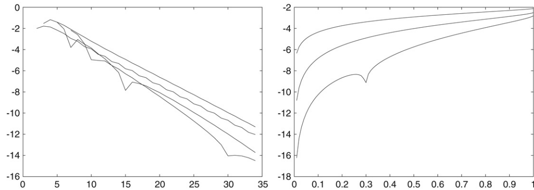
Fig. 4. Left: \log_{10} of the error in the numerical computation of \delta_2 as function of the index n of F_n , using extrapolation of order from zero to three. Right: \log_{10} of the error in the adjustment of \Delta(\varepsilon) by its constant, linear and quadratic Taylor polynomial.
