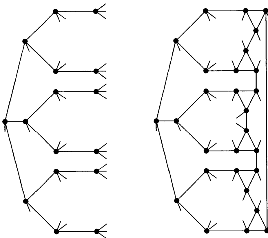
Figure 3: Modification of H_3 that gives H_3(K_3)
