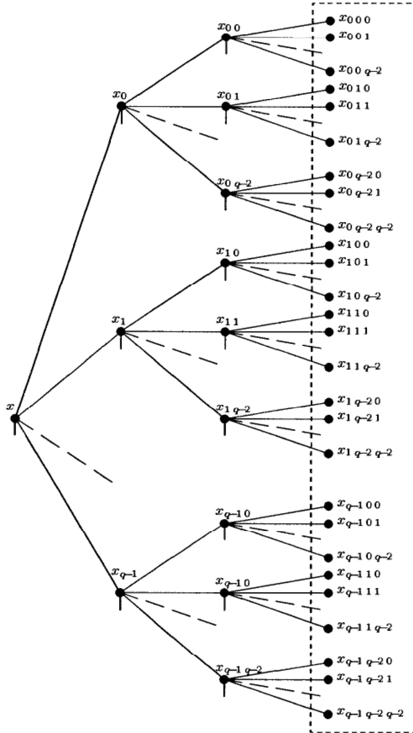
Figure 1: The subgraph of H_q to be modified.
