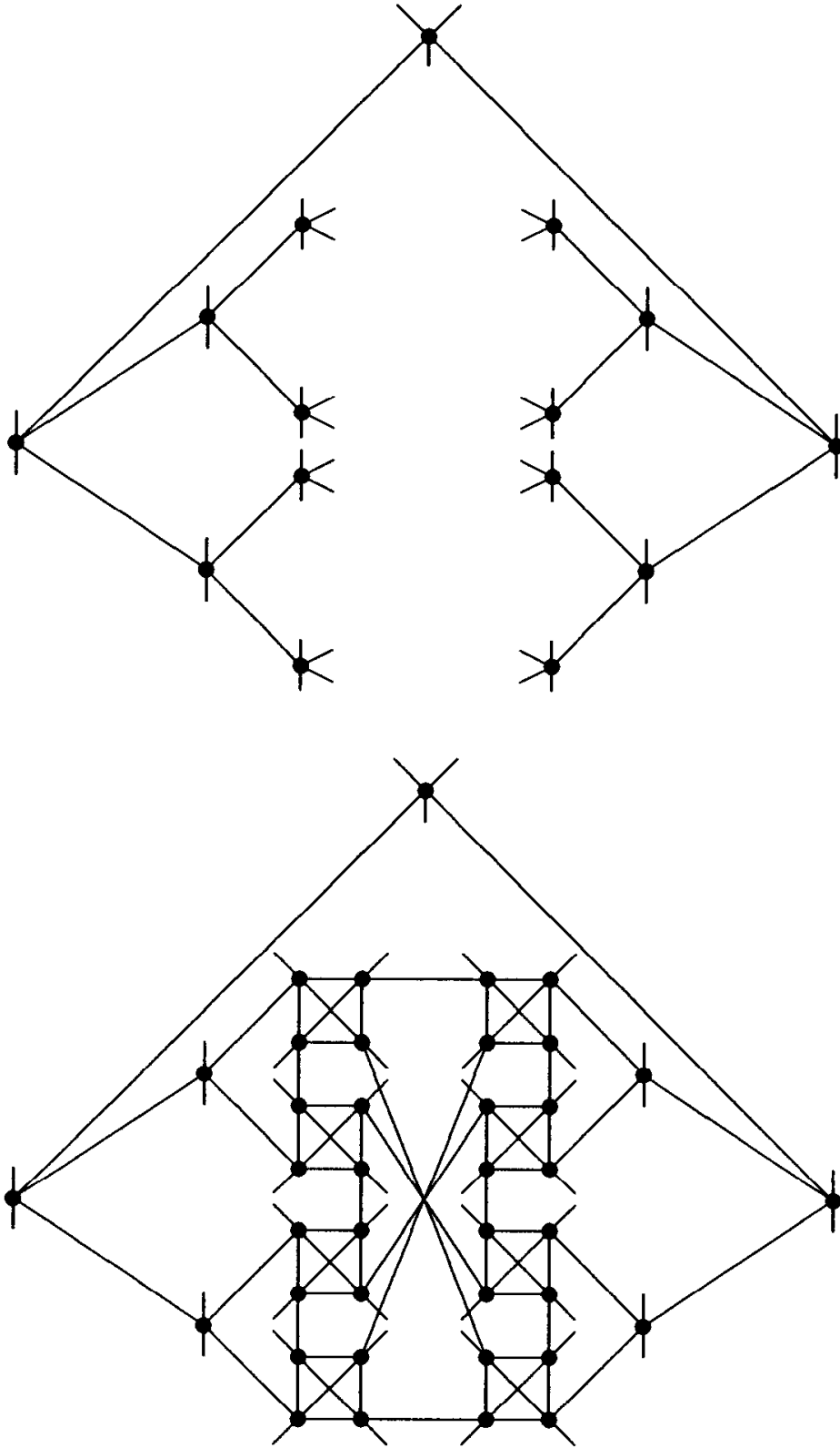
Figure 4: Graph H_5(K_4) with 7860 vertices.
