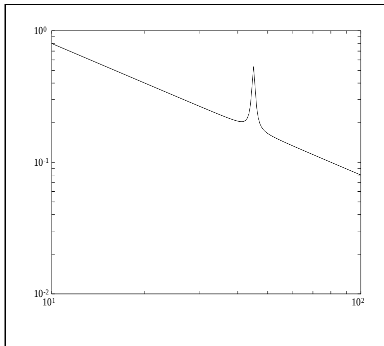
Figure 7.6: Loopshape, Example 3.
