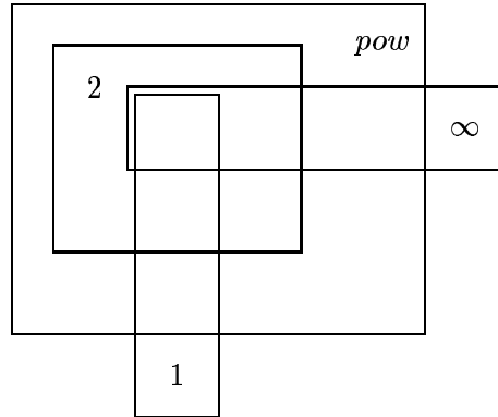
Figure 2.1: Set inclusions.
