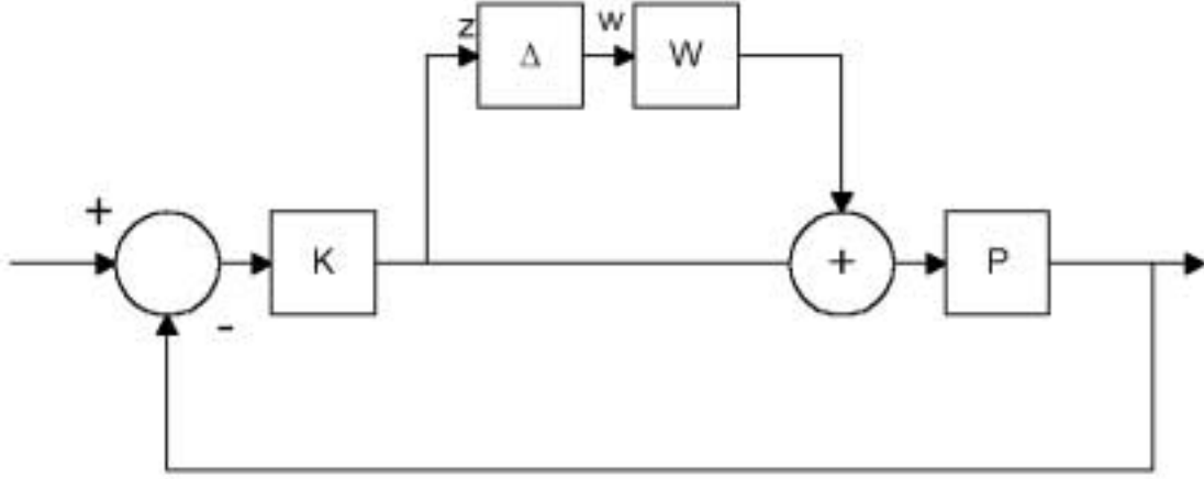
Figure 1: 20.1 Block Diagram.
