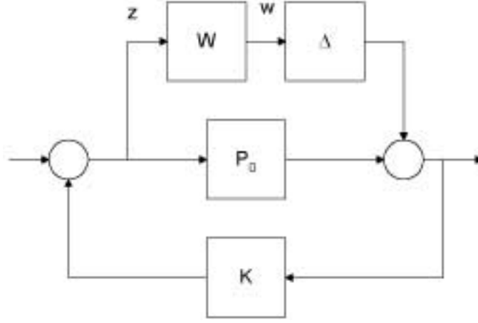
Figure 5: 21.1 Block Diagram.
