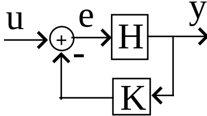
Figure 2: Feedback with positive definite gain matrix K > 0 .
