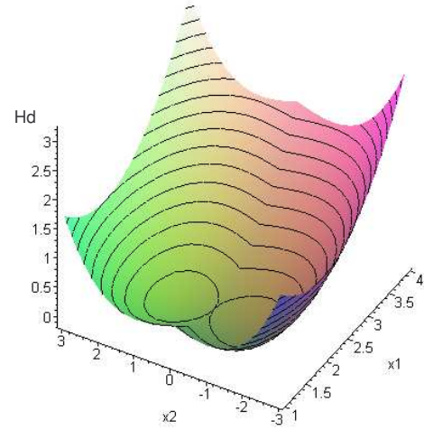
Fig. 1. Desired Hamiltonian function, H_d .
