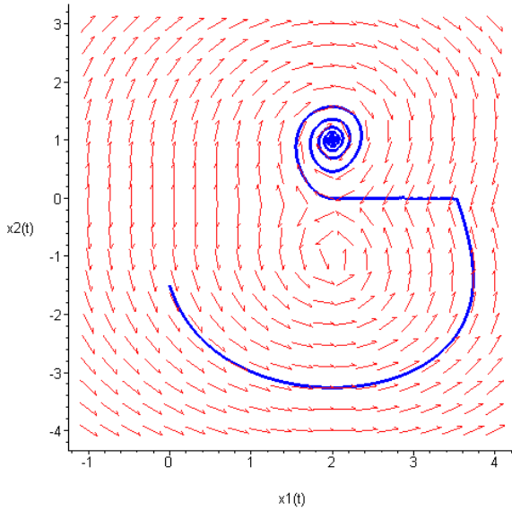
Fig. 4. State space; trajectory and vector field.
