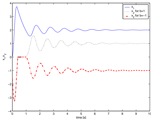
Fig. 6. Simulations for two different b values.
