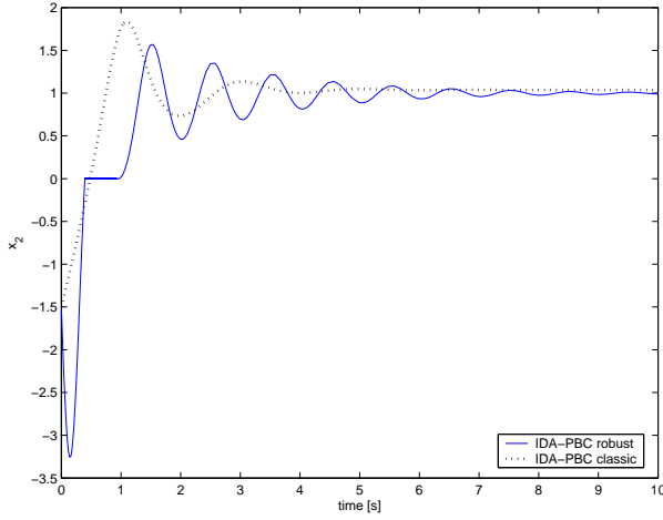
Fig. 3. Comparison between the robust method and the classic IDA-PBC, behaviour of x_2 .
