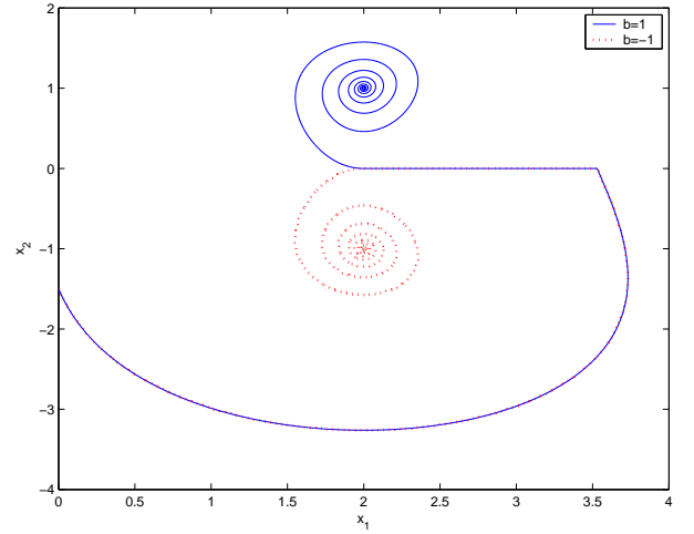
Fig. 5. Phase portrait of x for two different b values. b = 1 with a continuous line and b = -1 with a dotted line.
