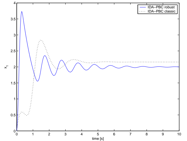
Fig. 2. Comparison between the robust method and the classic IDA-PBC, behaviour of x_1 .
